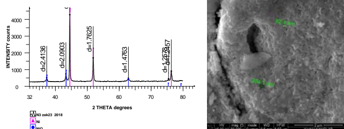
Figure 1 – XRD-pattern and SEM image of a Ni/NiO sample
