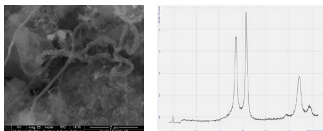
Figure 2 - SEM image and Raman spectra of carbon nanotubes at different scales synthesized on Ni/NiO@sp-Al 2 O 3
